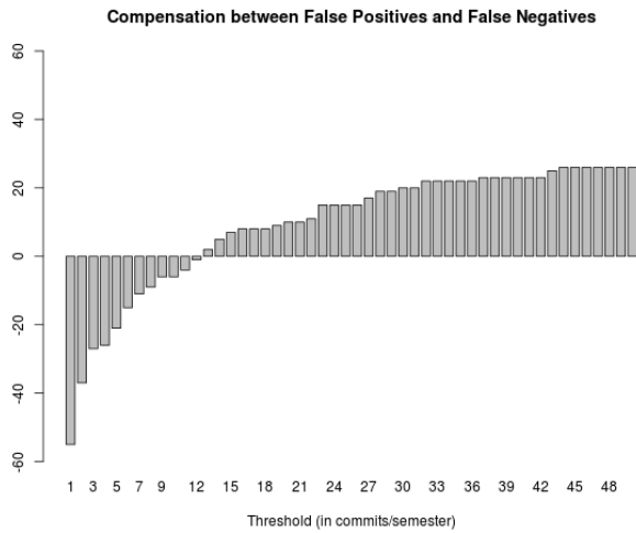
Figure 5: Compensation between false positives and false negatives for values of t . Negative values of the y axis indicate false positives that do not get compensated by false negatives, while positive values of the y axis indicate false negatives not compensated by false positives.
