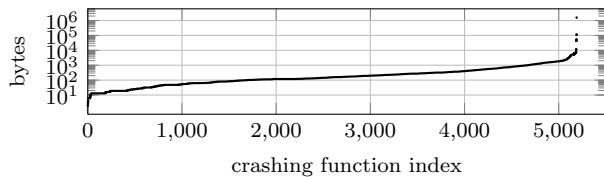
Figure 4: Function size for unique oopses containing both a code snippet and function name
