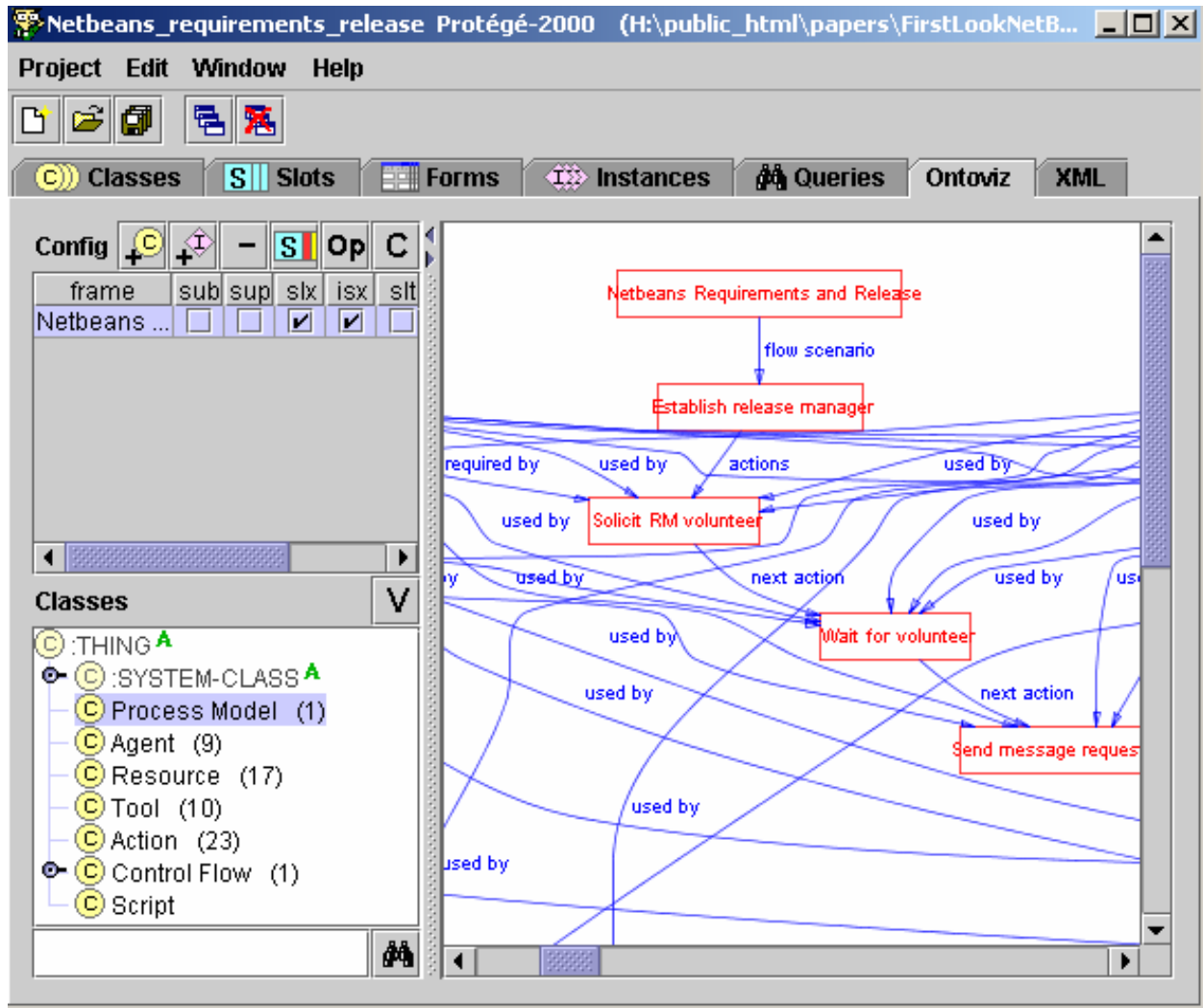
Figure 4. A view of the process domain ontology for the NetBeans.org software requirements and release process.
