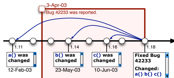
Figure 2: Locate fix-inducing changes for bug 42233
