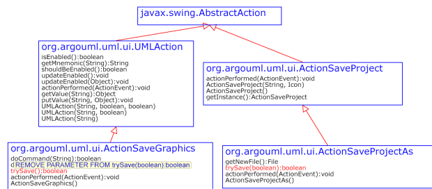
Figure 3: Missing Remove Parameter refactoring.
